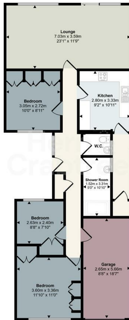
Floorplan
